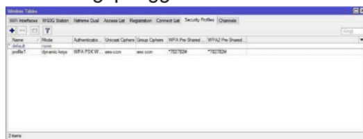
Gambar 15 Security Profile
