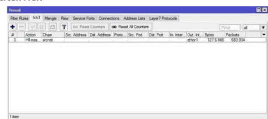
Gambar 13 Firewall NAT Router Kelas
