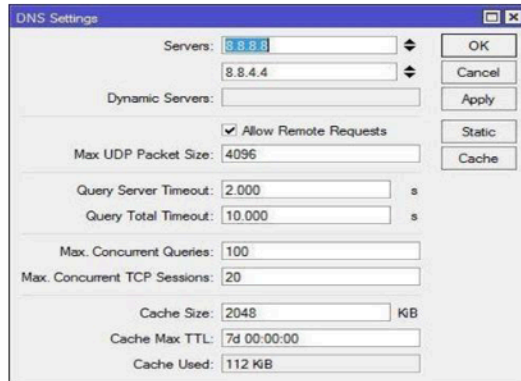
Gambar 7 DNS Server
