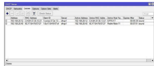
Gambar 22 Leases
