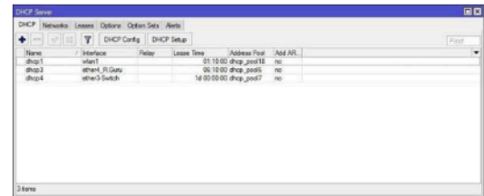
Gambar 10 DHCP Server
