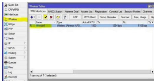
Gambar 14 Wireless Interfaces
